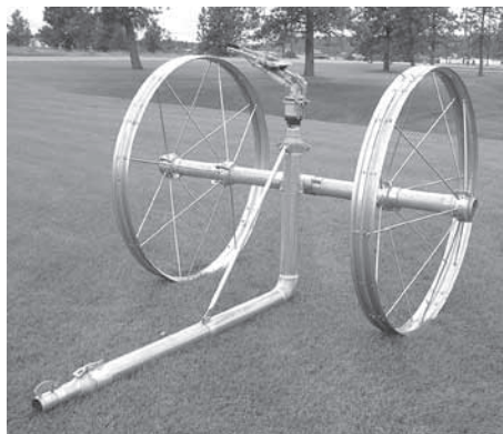
Big Gun® Cart Assembly recommended for use with Nelson 100 Series Big Gun® Sprinkler or equivalent.
