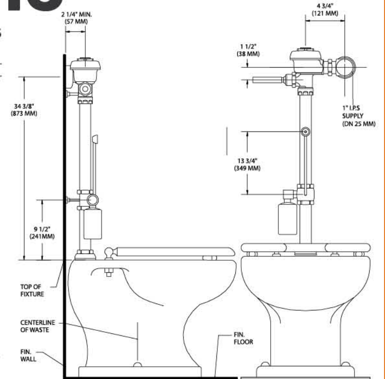
BPW-1005-1.6 Fluxómetro
