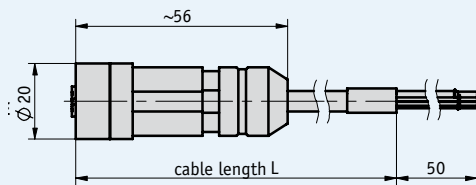
Type of connection GE
