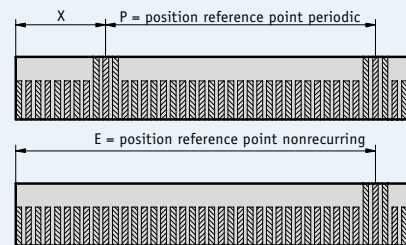
Reference points (all details in mm)
