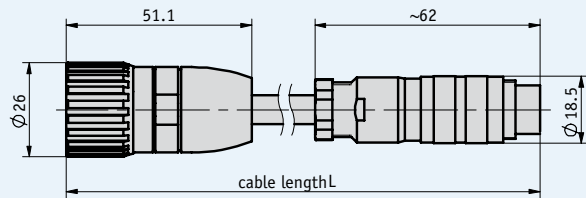
Type of connection GE/GE
