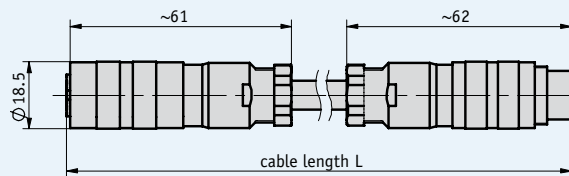
Type of connection GE
