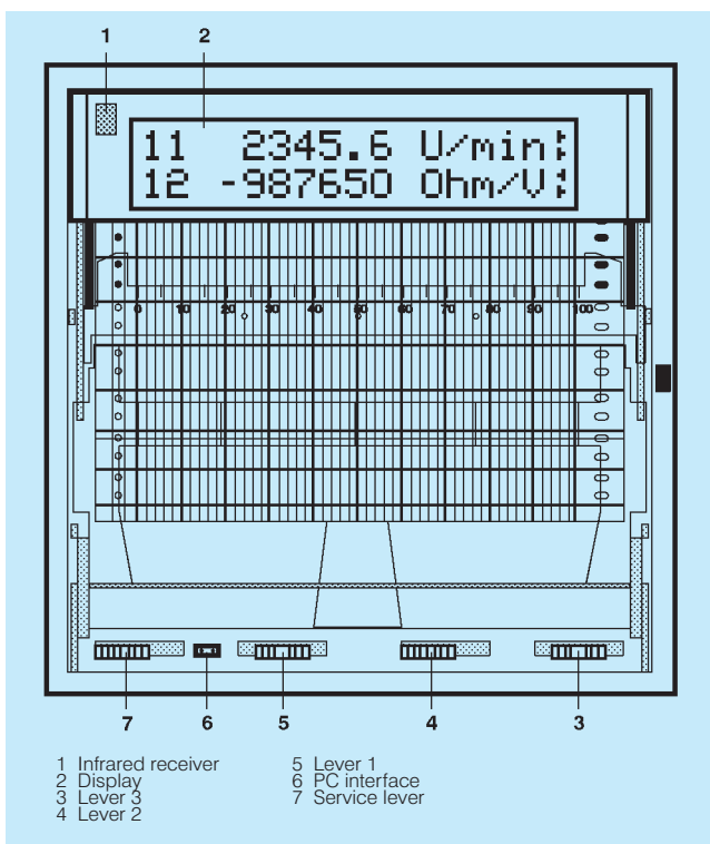
Fig. 2/15 Front view
