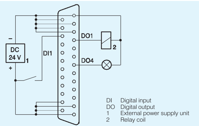
Fig. 3/15 Digital input/output, connection example
