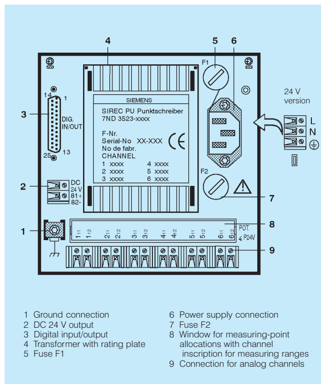
Fig. 2/16 Rear view
