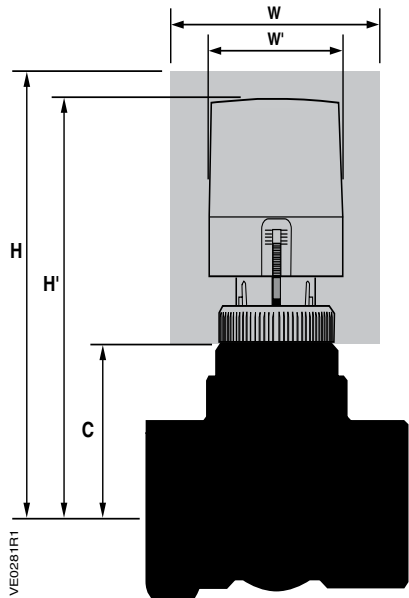
Thermic Actuator: 2-way Valve Assembly Service Envelope
