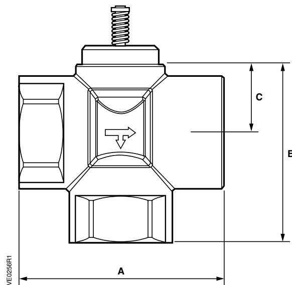
Three-way Zone Valve Body
