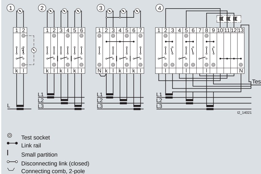
Connection possibility for measuring transformer terminals (instrument sets)
