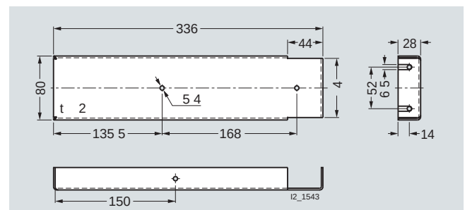
Side support (8HP9 045)
