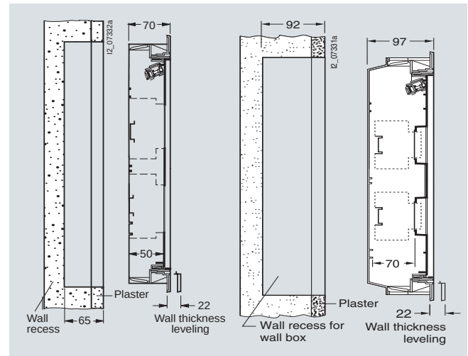
Device mounting depth 55 mm (left) and 70 mm (right)
