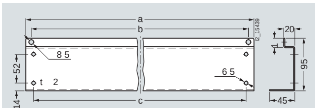
Joining sheet (8HP9 046)
