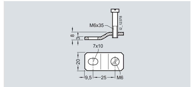
8HC3 800 fixing lug for individual enclosures and small distribution boards
