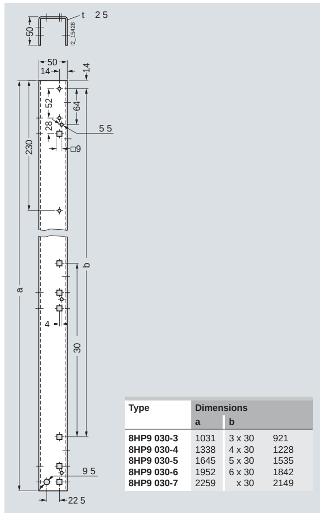
Support profile (8HP9 030-.)
