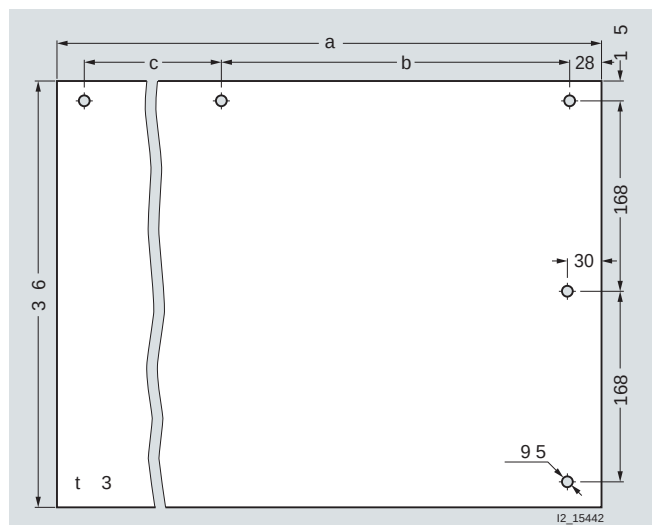
Cover, top (8HP9 073-.)
