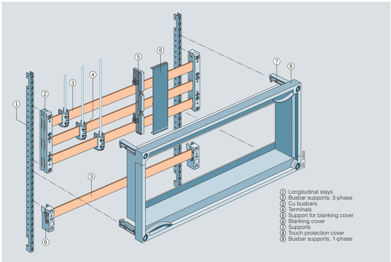
Distribution board components
