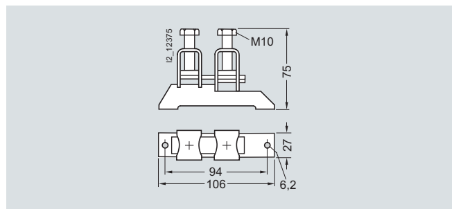
8JK4 04
