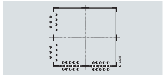
Enclosure size 4
