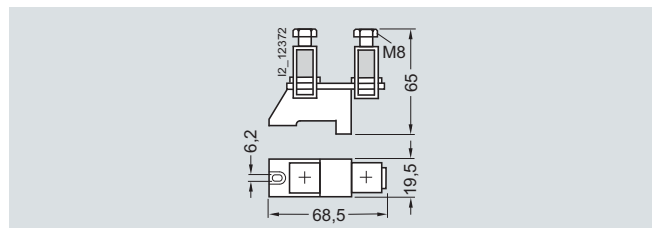
8JK4 01
