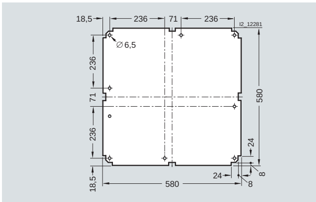
8HP6 304 for encl. size 4, sheet steel, 2 mm thick, sendzimir-galvanized
