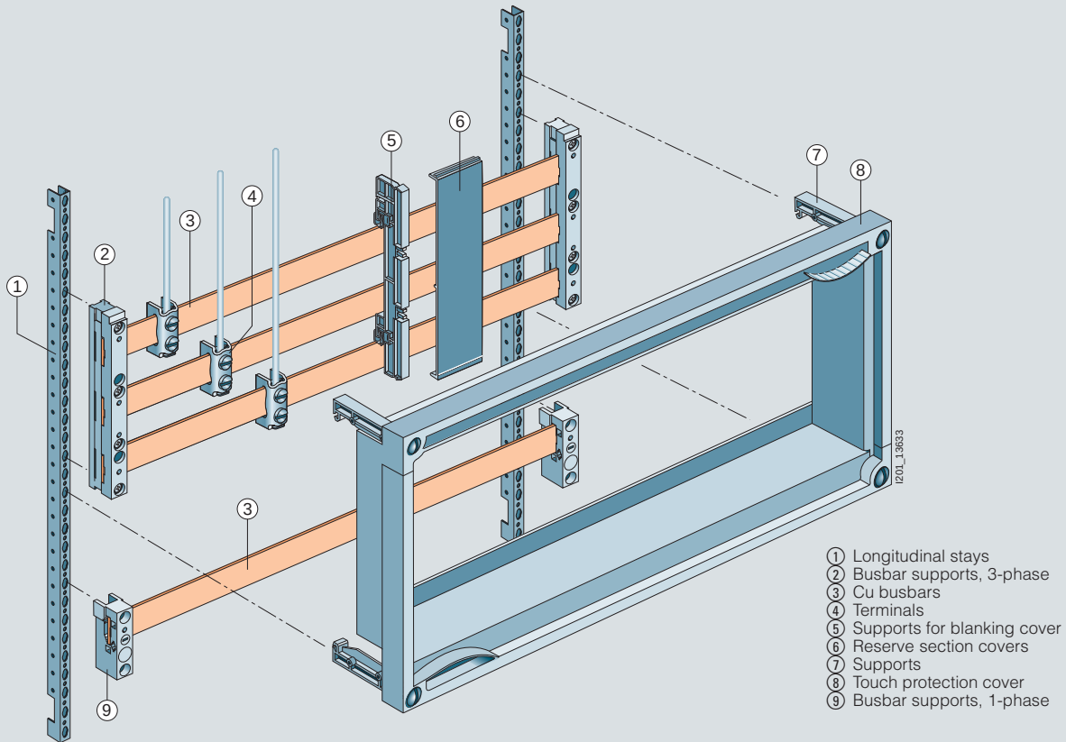
Distribution board components
