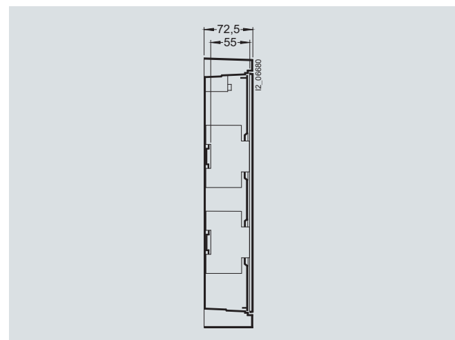
Device mounting depth: 55 mm
