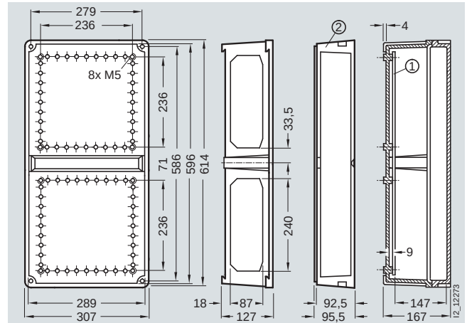
Enclosure size 3
