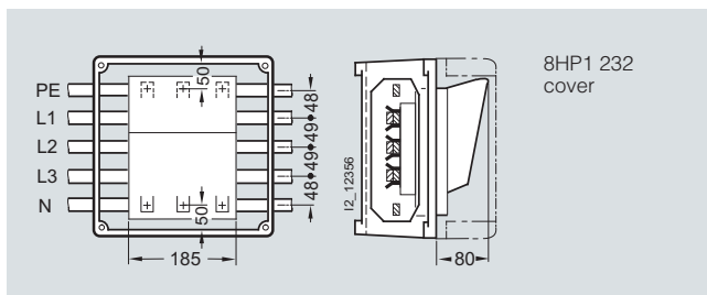
Busbars 400/630 A for 8HP4 314 switch
