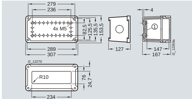
Enclosure size 1
