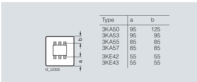
Enclosure size 2
