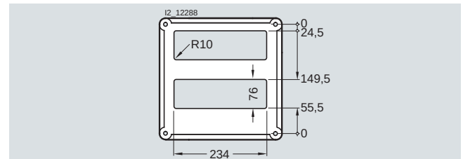
8HP1 352 for enclosure size 2
