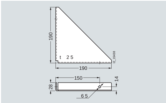
Joining sheet (8HP9 046)
