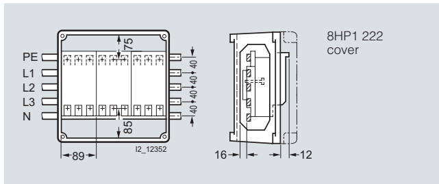
Busbars 250 A for 3NP40 1 switch
