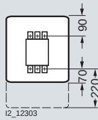
8HP2 440 or 8HP2 441, with 2 or 3 fuse switch disconnectors
