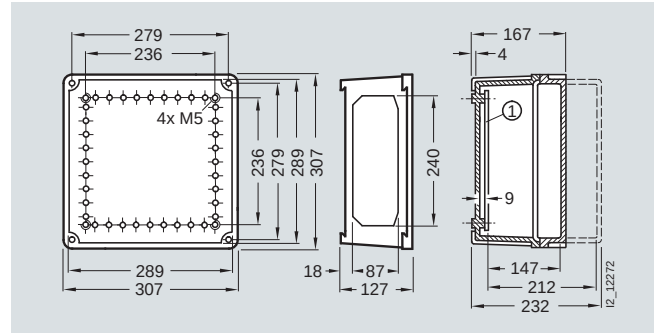
Enclosure size 2
