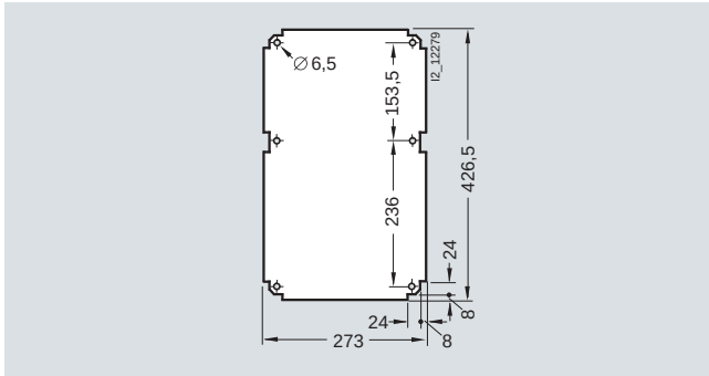
8HP6 307 for encl. size 2.5, sheet steel, 2 mm thick, sendzimir-galvanized
