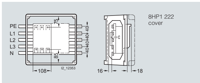
Busbars 250 A for 3NP40 7 switch
