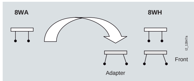
Adapters for inscription of 8WA8 front labels
