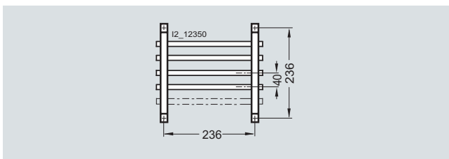
8HP1 790 for enclosure size 2
