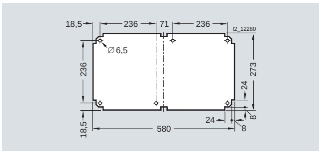
8HP6 303 for encl. size 3, sheet steel, 2 mm thick, sendzimir-galvanized
