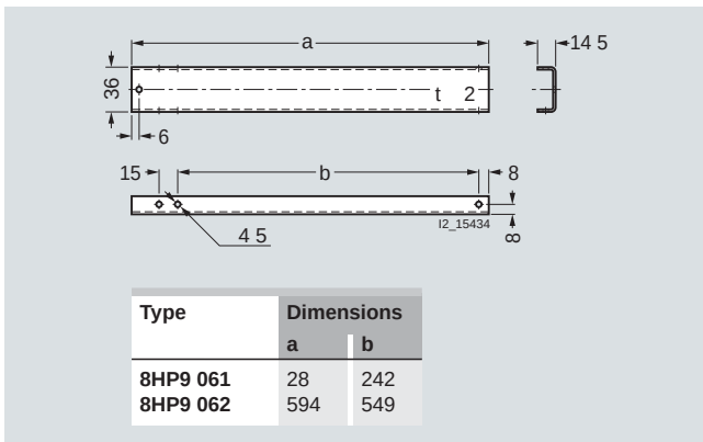
Corner profile (8HP9 061, 8HP9 062) with connecting bracket
