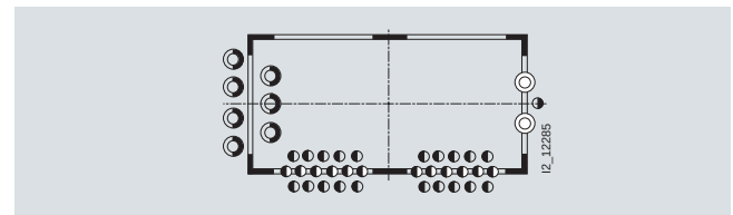
Enclosure size 3
