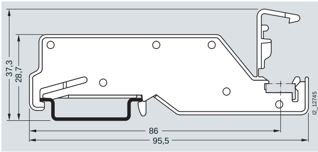
8WH 140-0CA00
