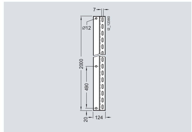
8HP9 020 wall-mounting bracket
