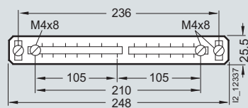
8JH1 41 to 8JK1 13 for meters, time switches and timing relays
