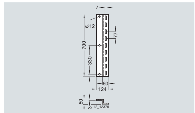
8HC3 510 wall-mounting bracket
