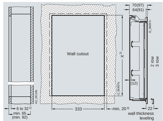
Device mounting depth 55 mm (dimensions in parentheses apply to mounting depths of up to 70 mm)
