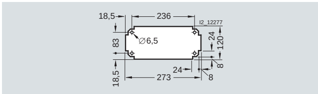
8HP6 301 for encl. size 1, sheet steel, 2 mm thick, sendzimir-galvanized
