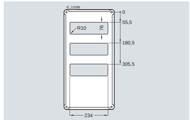
8HP1 353 for enclosure size 3
