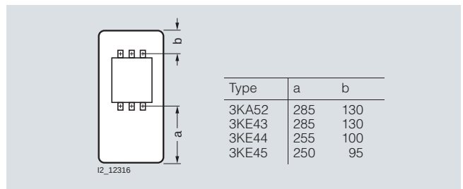
Enclosure size 3
