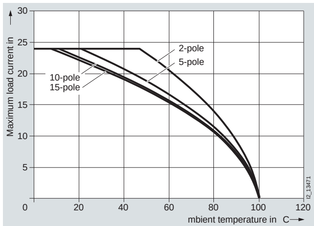
Derating curve for 8WH5 100-2KF00 and 8WH5 103-2LF00
