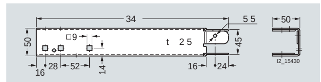
Support profile extension (8HP9 034)
