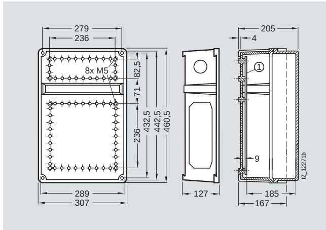
Enclosure size 2.5
