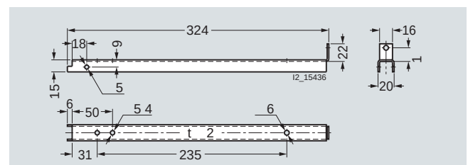
Support strut (8HP9 067)
