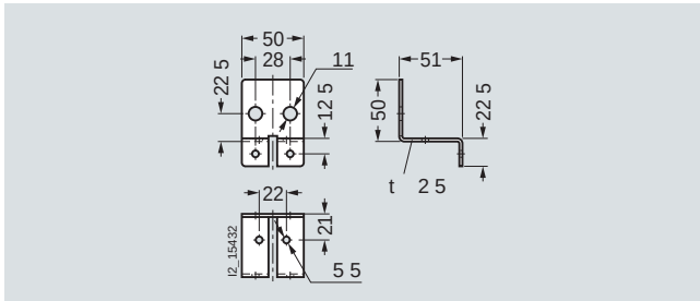
Connecting bracket (8HP9 060)
