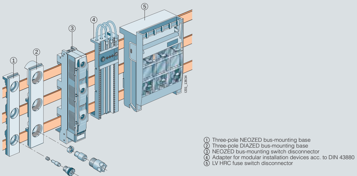
Built-in components
