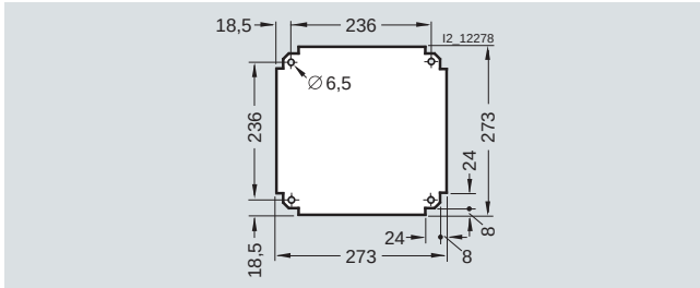
8HP6 302 for encl. size 2, sheet steel, 2 mm thick, sendzimir-galvanized
