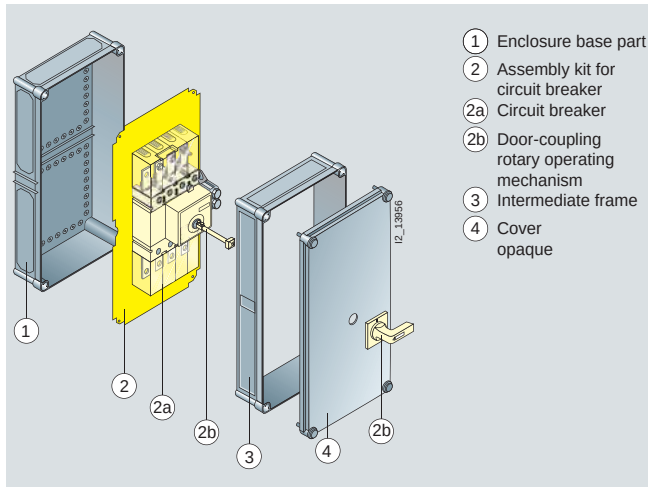
ALPHA 8HP, diagram of enclosure with 3VL circuit-breakers
