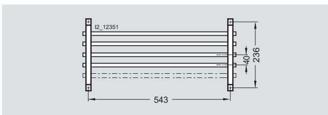
8HP1 791 for enclosure size 3
