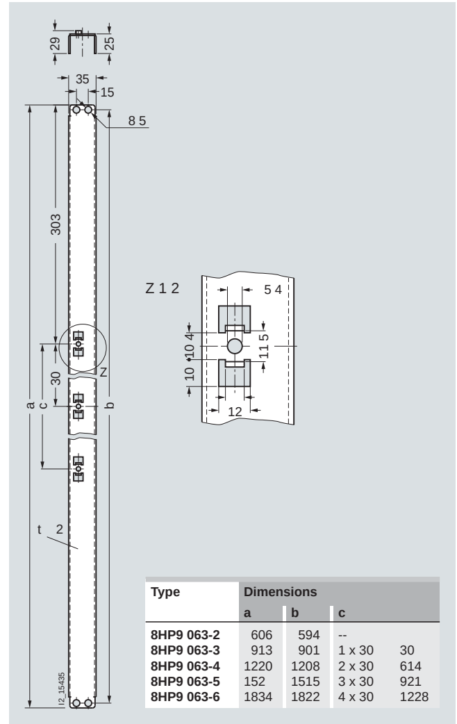
Lateral profile (8HP9 063-.)
