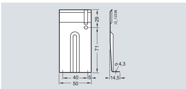
8HP6 201 holder for mounting measuring instruments
