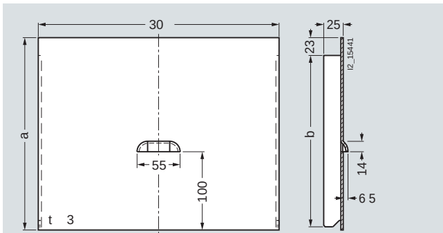
Baseboard (8HP9 038-.)
