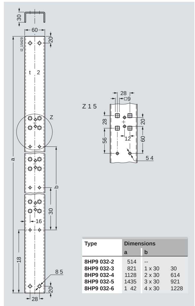
Support rail (8HP9 032-.)
