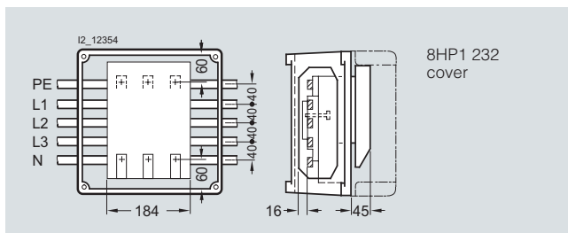
Busbars 250 A for 3NP42 switch
