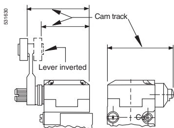
Figure 4—Cam track dimension
