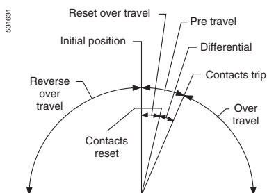
Figure 5—Contact travel
