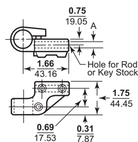
Adjustable Length Rod Type
