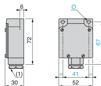
Body mountings
