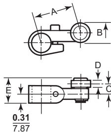
Type T and FT Lever Arms Standard Roller
