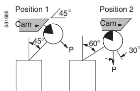
Figure 1A cam design for speeds up to 50 fpm
