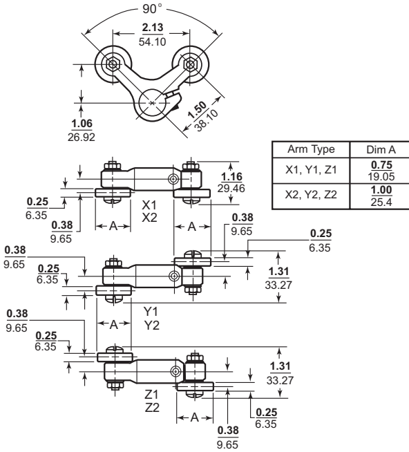
Type T and FT Lever Arms (continued) 90° Forked
