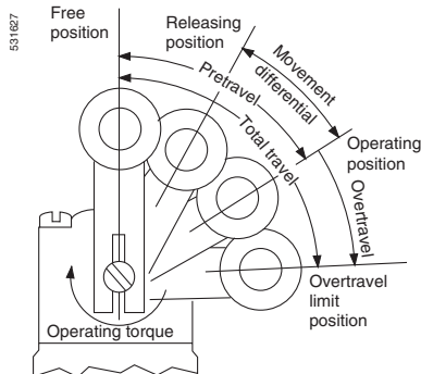
Figure 1: Rotary lever type
