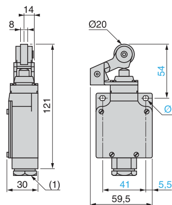
Body mountings
