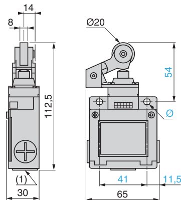
Rear view XCKM•••, ZCKM•, ZCKMD3•
