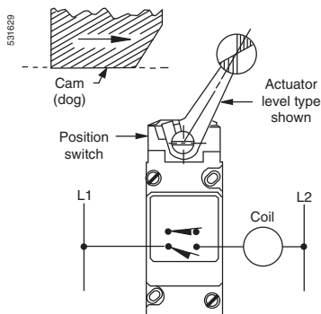
Figure 3—Limit switch
