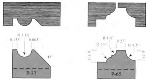
DRAWINGS NOT TO SCALE
