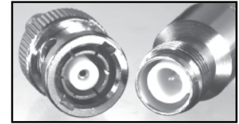
Reverse Polarity BNC male and Reverse Polarity TNC female
