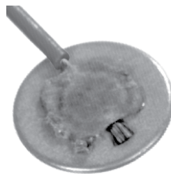
Weld of copper wire to plastic electrode. (Shown at 300% size)
