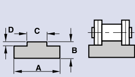
PLASTIC GUIDE RAILS HORIZONTAL - T-PROFILE
