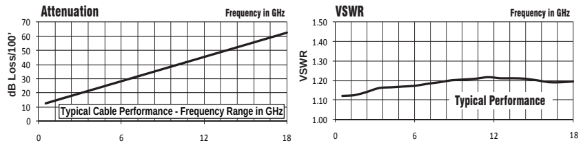
Typical Plot for PE39423-12
