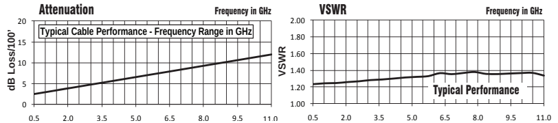
Typical Plot for PE39451-12
