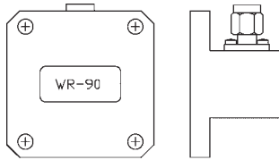
WAVEGUIDE TO SMA TYPE MALE
