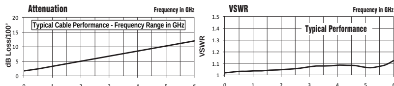
Typical Plot for PE39479-12
