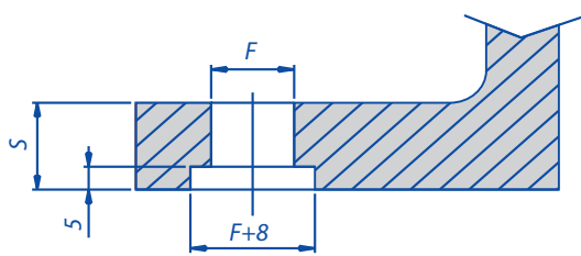
Fig. 5: Flange fixing holes
