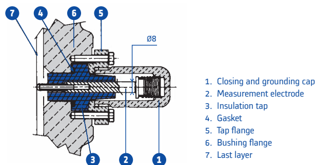
Fig. 2: Power Factor Tap
