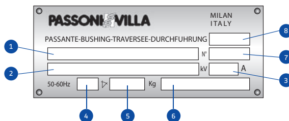
Fig. 4: Nameplate
