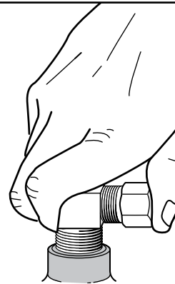
Finger Tight
