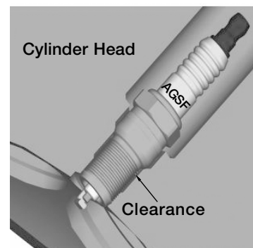
“FULL THREAD” AGSF-type
