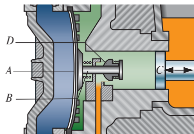
Figure 3 Diaphragm (A) and piston (C) are full rearward, once again forcing Mars valve (B) to its rearward position, which allows poppet (D) to open if required. Low oil volume creates a vacuum and opens poppet, permitting hydraulic fluid to enter the chamber from the refill line.
