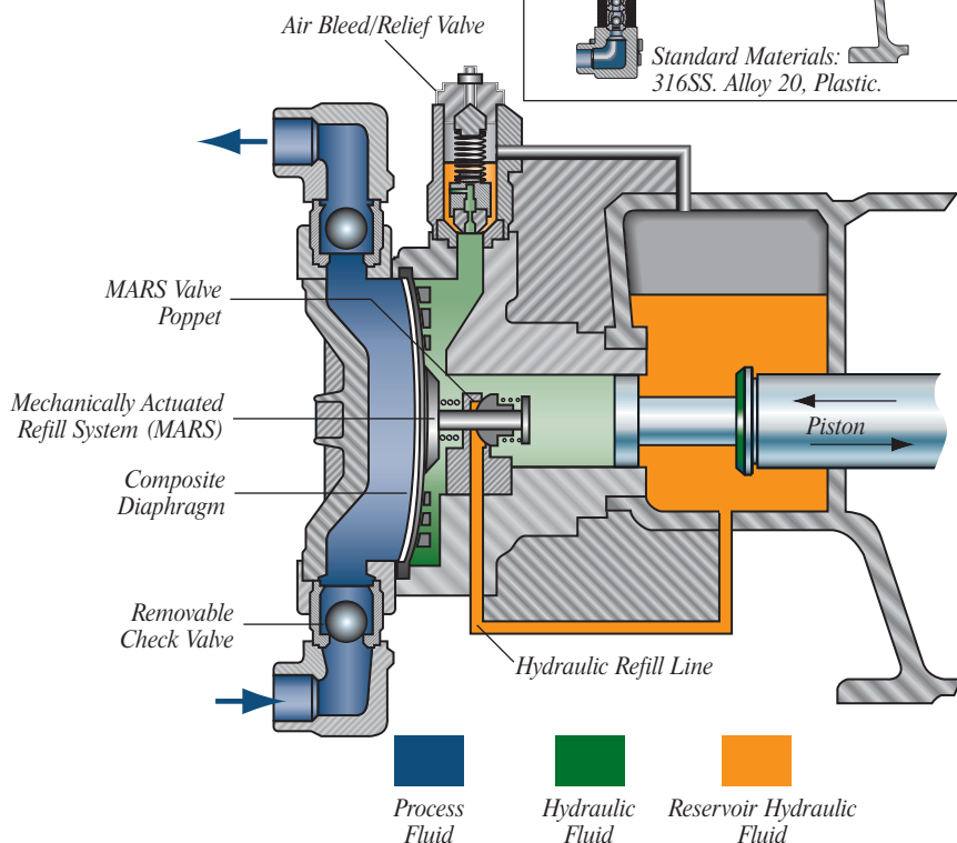
Full side view of HPD Liquid End on MilRoyal Drive
