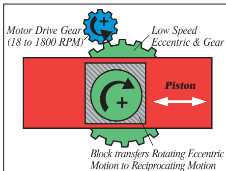
CENTRAC Scotch Yoke Drive
