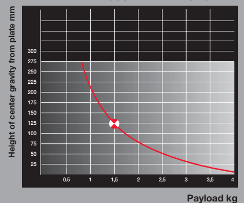
COUNTERBALANCE GRAPH
