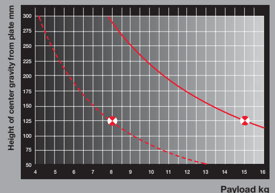
COUNTERBALANCE GRAPH
