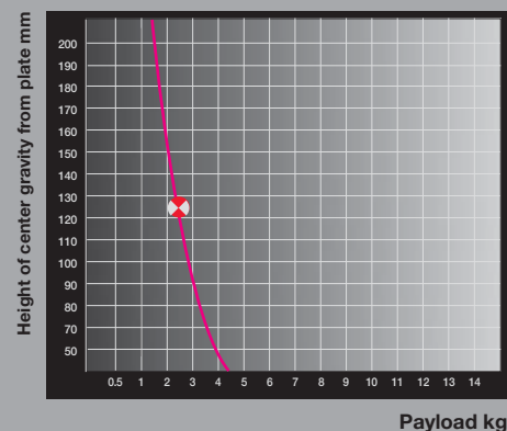
COUNTERBALANCE GRAPH
