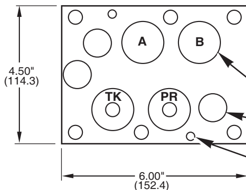
Pocket for 1 5/16" O.D. O'Ring (4) Places
