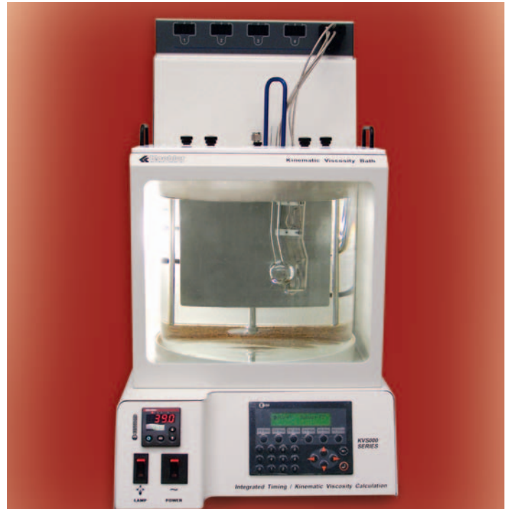
K23702-OS Kinematic Viscosity Bath (KV5000) with K23780-CF Optical Sensor and CF Routine Tube 378-025-C02-OS
