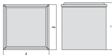
IP65 Aluminium enclosure
