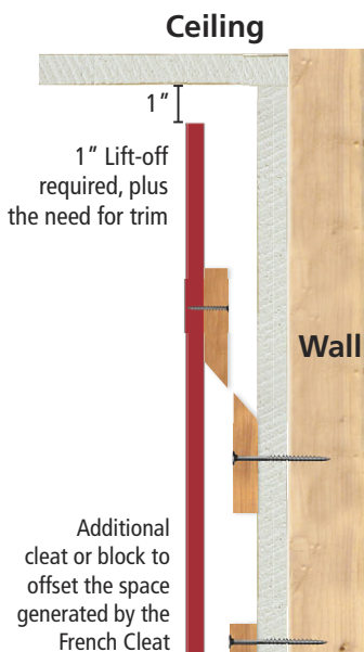
French Cleat
