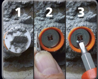
Capped, Uncapped, Removed
