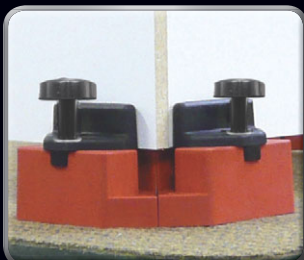
The Ass. Block holds all your parts in place
