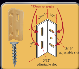
Nylon Kolbe Korners
