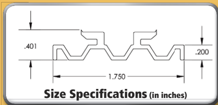
SmartCleaT™
