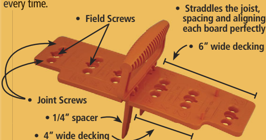
Straddles joists for a secure fit and even spacing between boards
