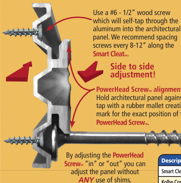
French Cleat
