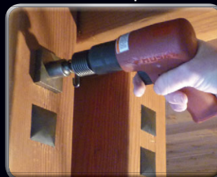
The 2" Artisan Chisel on an air hammer leaves a perfect outline for the Accents.
