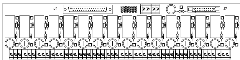
J1= SUB-D 37 Maschio SUB-D 37 Ways male
