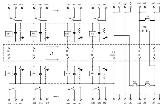
J1= SUB-D 37 Femmina SUB-D 37 Ways female
