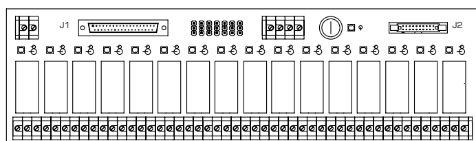
J1= SUB-D 37 Maschio SUB-D 37 Ways male
