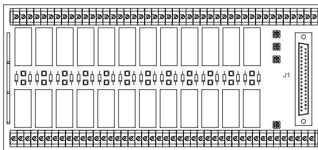
J1= SUB-D 37 Femmina SUB-D 37 Ways female
