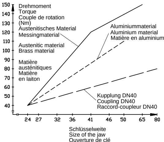
DILO-Anschluß DILO connection Raccord DILO
