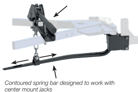
Adjuster slides on frame to avoid gas bottles and battery trays; slides adjust 18 to 28 inches
