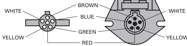
TRAILER END As viewed from front face of 6-way connector with molded on cable.
