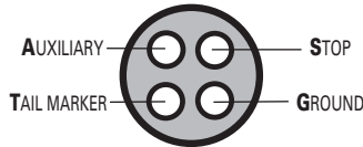
TRAILER END As viewed from core back side where wires are attached with screws.
