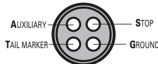
CAR END As viewed from core back side where wires are attached with screws.
