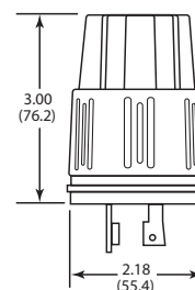
20 Amp Locking
