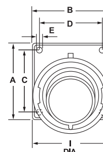
20, 30 Amp Front View
