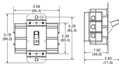
60002D, 60003D and 85002D, 85003D
