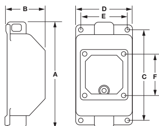
Feed-Through Box
