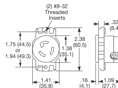
4712BRY and 4713BRY
