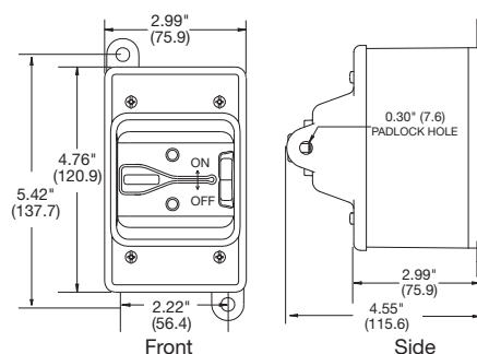
30322D and 30323D
