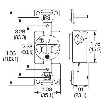
Single Receptacle Standard and Isolated Ground 8210
