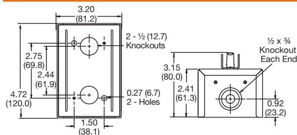
30102D and 30103D
