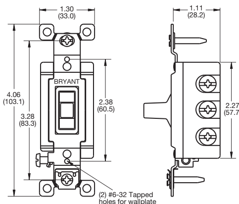
Double-Pole, Double Throw Switches
