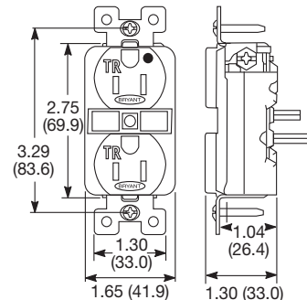
Tamper-Resistant Receptacle BRY8200TR
