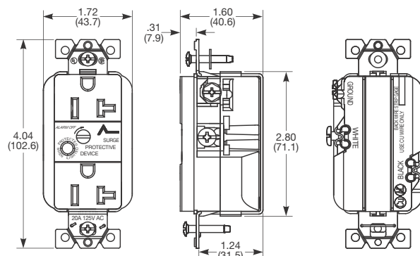
Surge Duplex Receptacle Series
