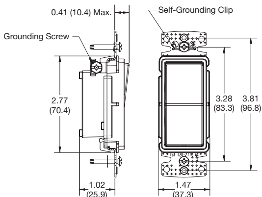
Single-Pole Decorator Switch
