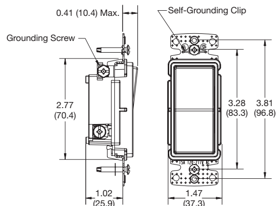
3-Way Decorator Switch
