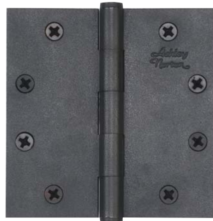
HIN4545 Shown in dark bronze patina 4 ½" x 4 ½" 0.134" thickness Supplied with #12 x 1 ¼" screws
