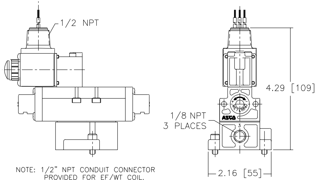
Constr. Ref. 3
