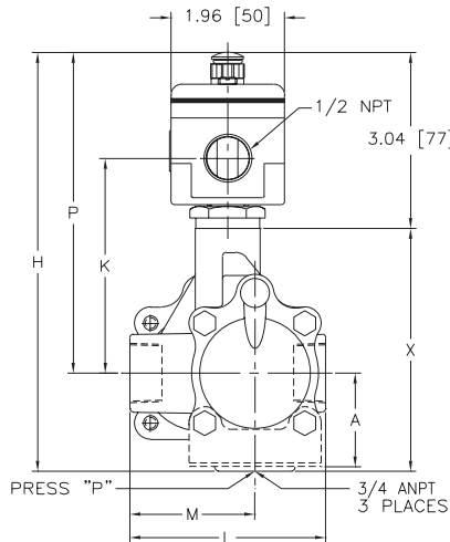
Constr. Ref. 7, 7A
