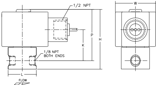
Constr. Refs. 2, 4, 6, 9
