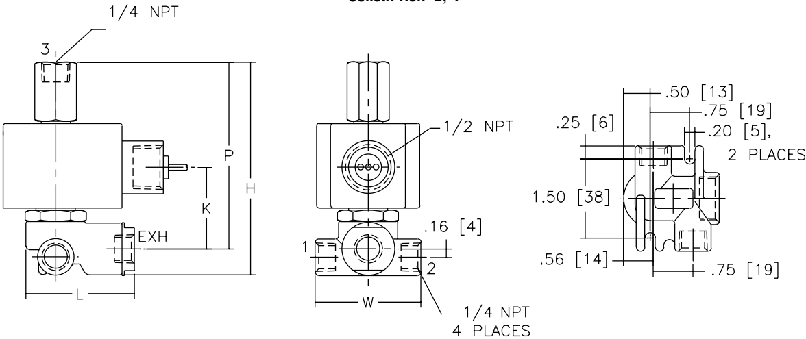
Constr. Ref. 2, 4
