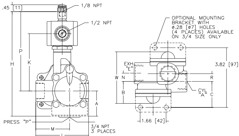
Constr. Ref. 8
