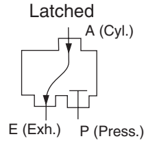
Flow Diagram C
