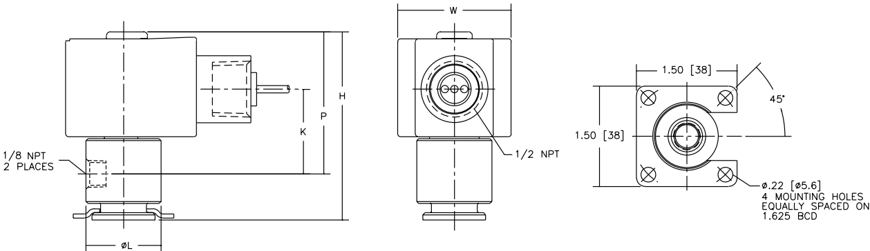
Constr. Ref. 8
