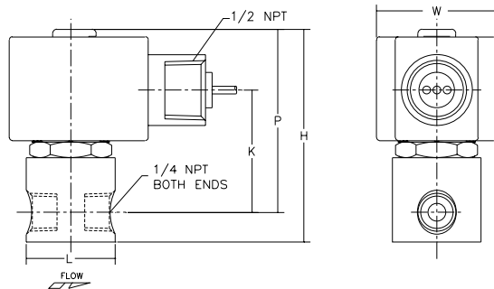
Constr. Refs. 11-14, 16, 17
