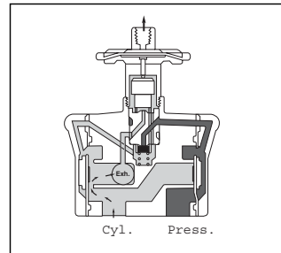
Figure 13A: Normally Closed, Operator Exhausted
