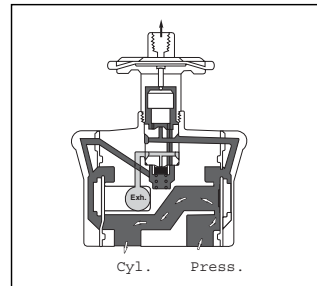
Figure 13C: Normally Open, Operator Exhausted
