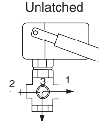
Flow Diagram B
