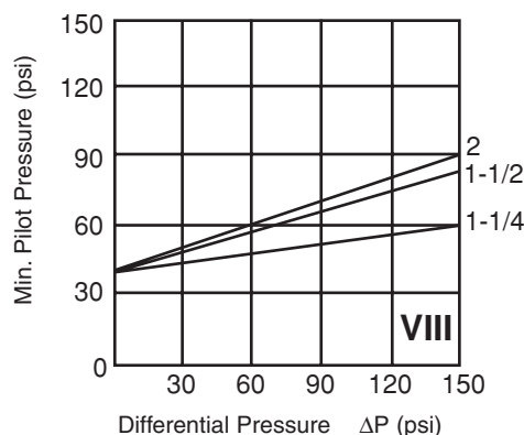
Normally Open
