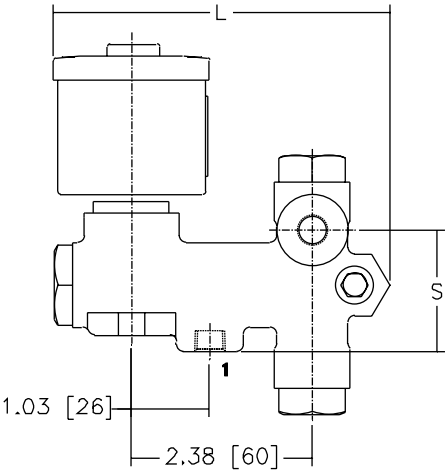
Constr. Refs. 1, 2, 3, 4
