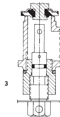
Threaded Stem in Body
