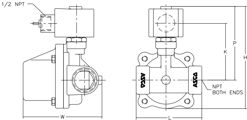
Constr. Ref. 8
