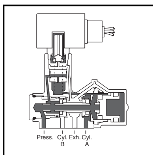
De-Energized
