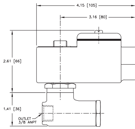
Constr. Ref. 2
