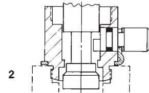
Rotary Stem in Bonnet
